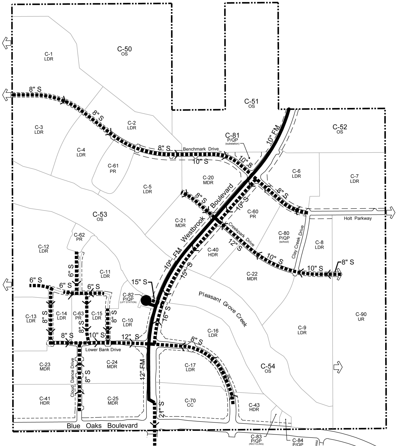
Figure 8-3: Wastewater Collection
