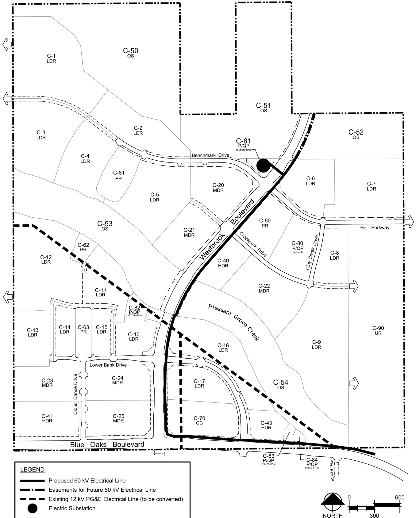
Figure 8-6: Electric Facilities
