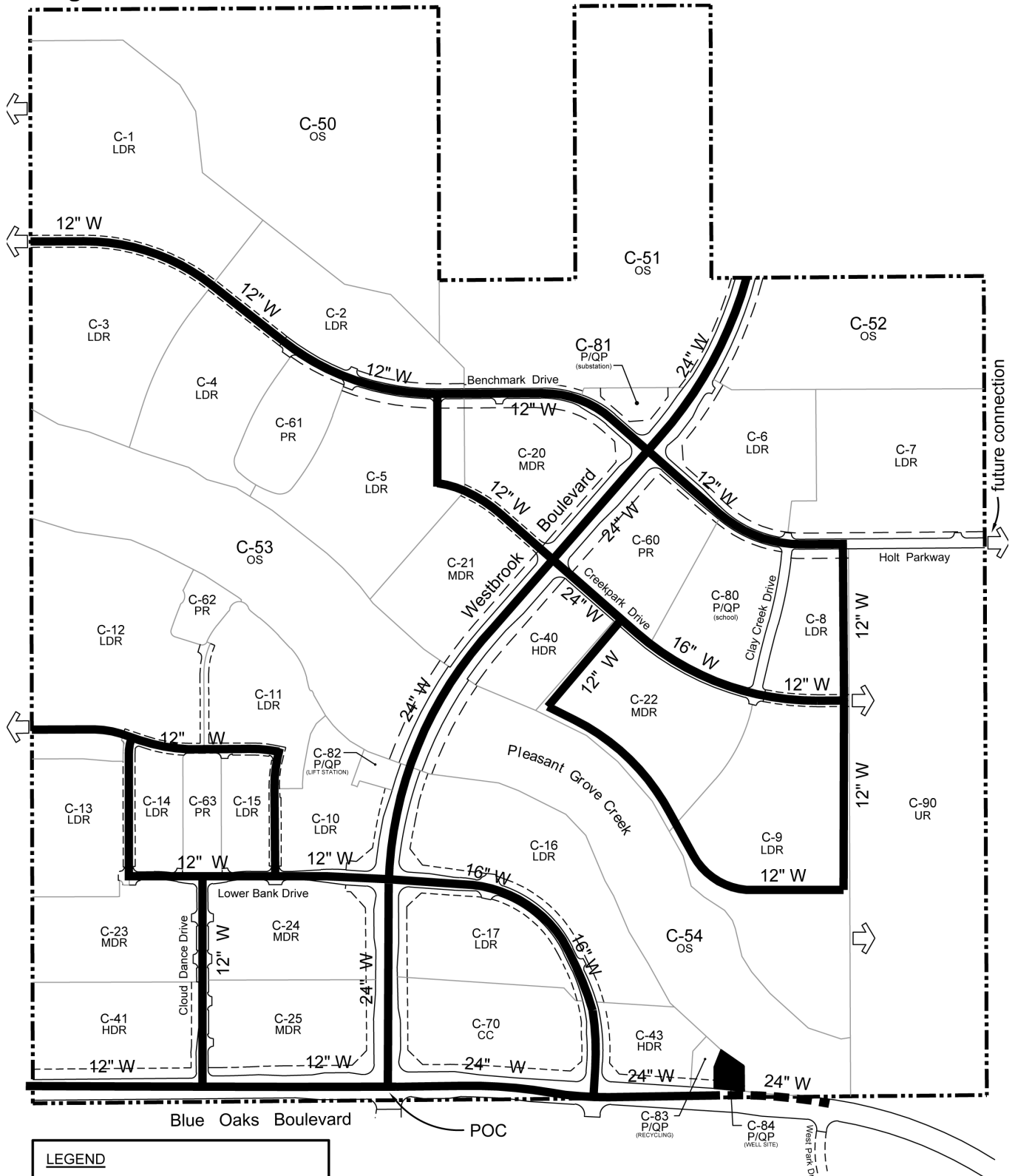
Figure 8-1: Water Facilities
