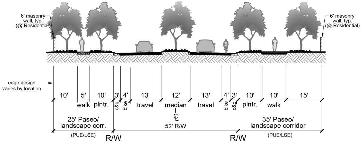
Figure 6-10 Lower Bank Drive Westbrook Boulevard to Blue Oaks Boulevard
