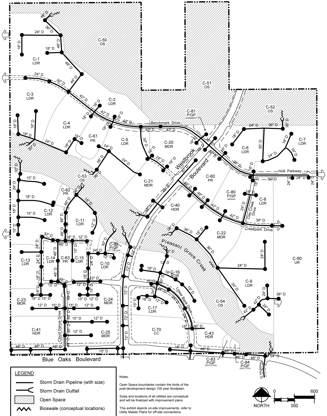
Figure 8-5: Drainage Improvements
