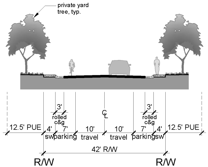
Figure 6-13a Minor Residential Street Attached Walk
